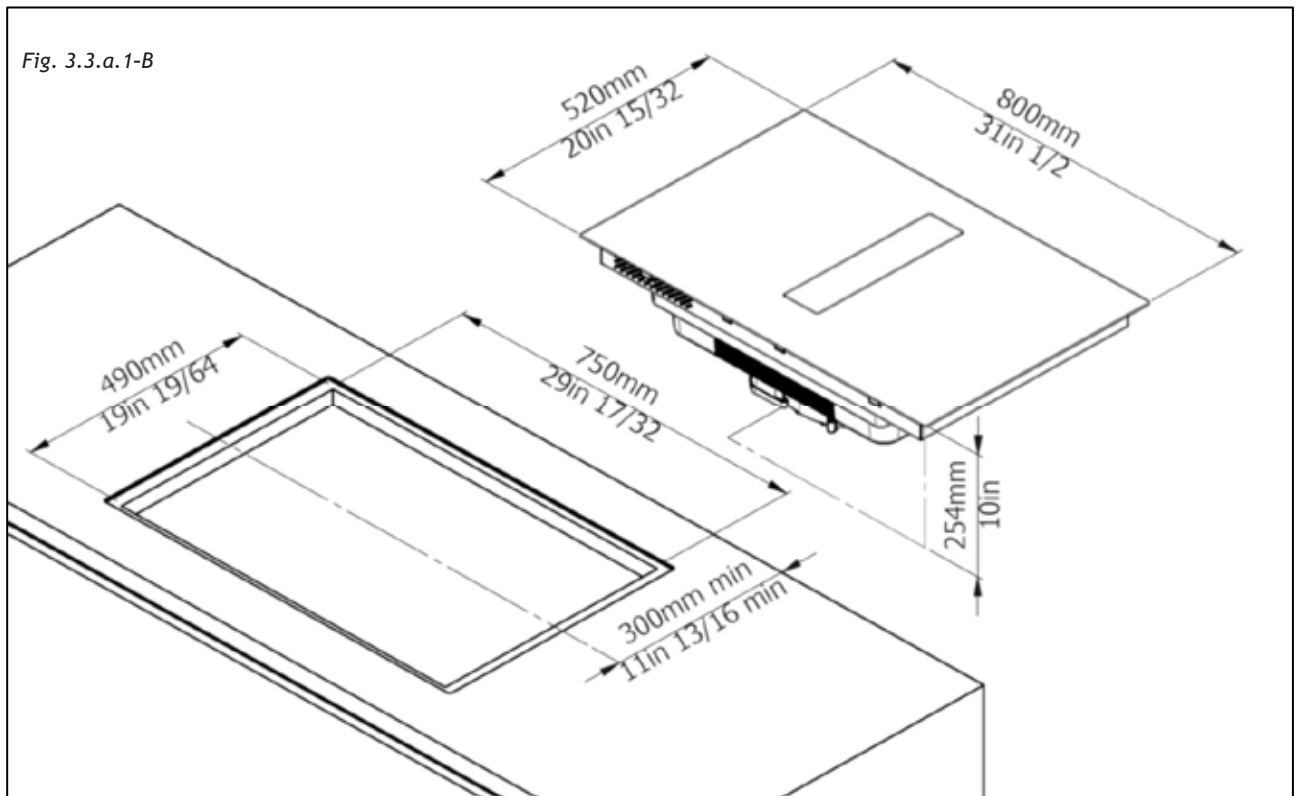
Fig. 3.3.a.1-B -> 80cm-31in 1/2 hob:
