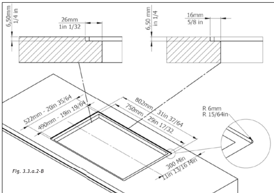
Fig. 3.3.a.2-B -> 80cm-31in 1/2 hob:
