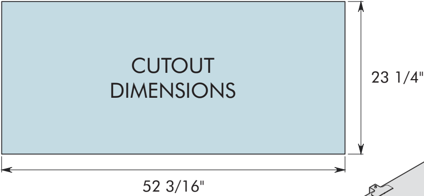
BOTTOM VIEW
