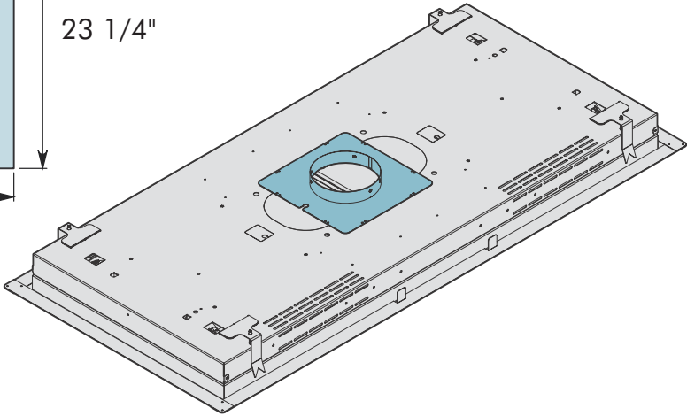
3D OVERVIEW
